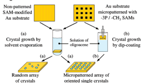
Scheme 1. Schematic Illustration of the Experimental Procedure for the SAM-Induced Growth of Organic Semiconductor Crystals from an Oligoacene/THF Solution 10
